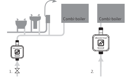
Figure 5: Typical installation locations
