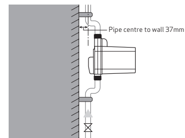
Figure 4: Modified pipe work for clearance
