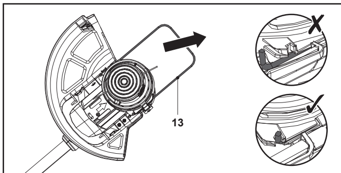
Fig. 12, trimming / edging position
