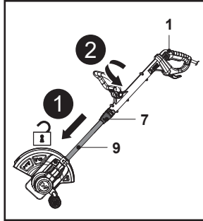
Fig. 9 A (initial position 90°)
