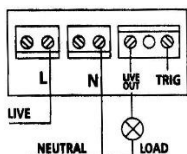
Figure 1: Standard Wiring
