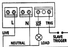
Figure 2: 3-Wire System
