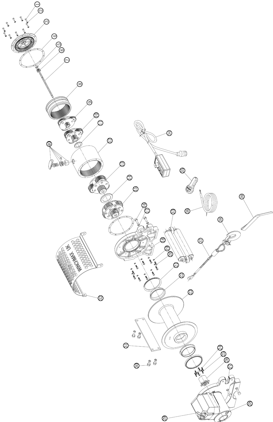
Parts Diagram 20,000lb Winch
