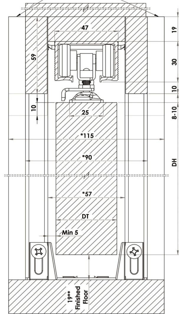
SECTION A-A 12.5mm Plaster Board
