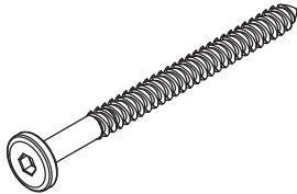
M7*90mm ST790*6
