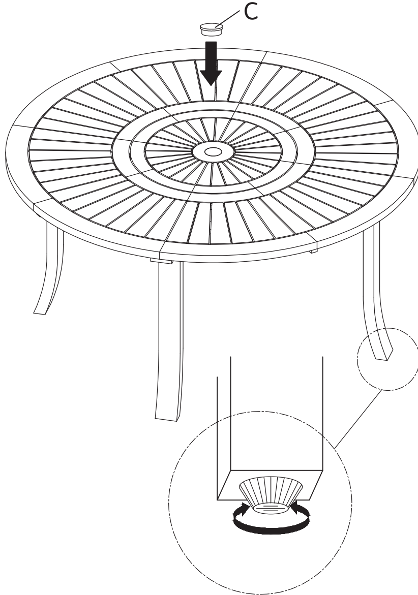
Levelling Screw
