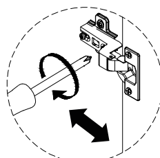
2. LATERAL ADJUSTMENT BY SCREW ADJUSTING
