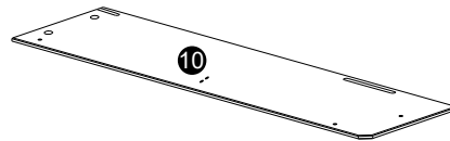
⑩ x1 760 x 190 x 12mm
