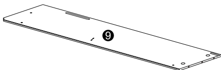
⑨ x1 760 x 190 x 12mm
