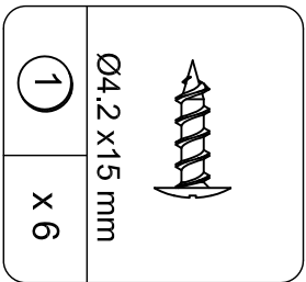
SCREW TCS1065
