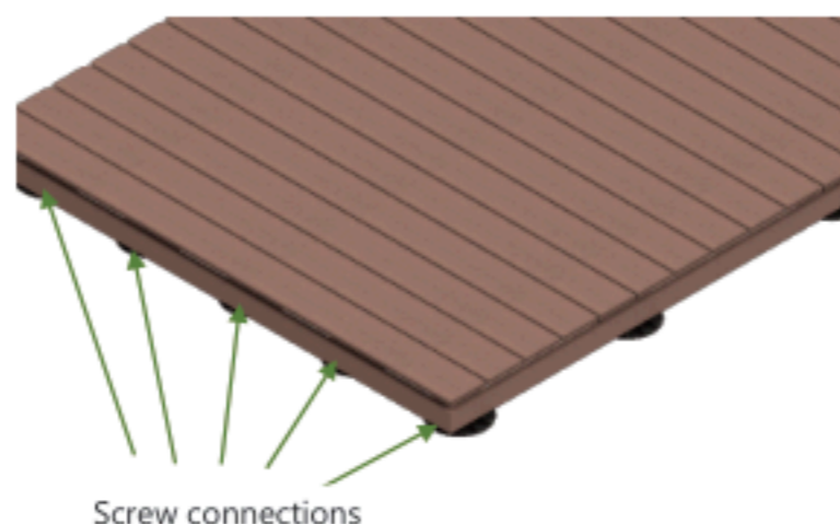
Screw connections
