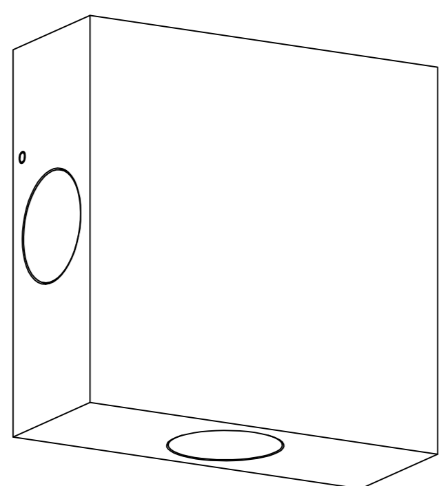
LWA-249 L130xW130xH50(mm) LED-4x3W
