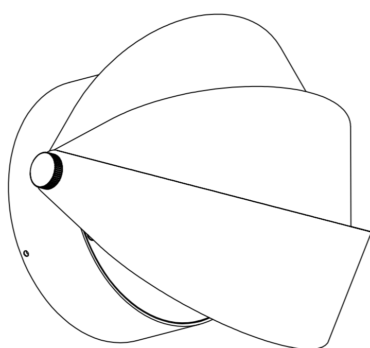
LWA-451 L176xW149xH178(mm) LED-6W
