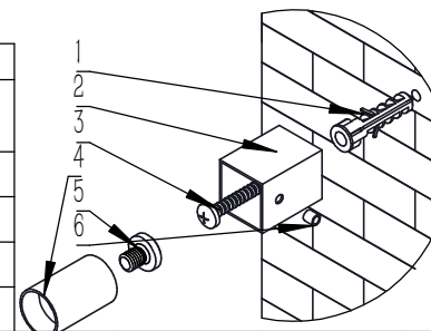
GRAB SCREW 4PCS
