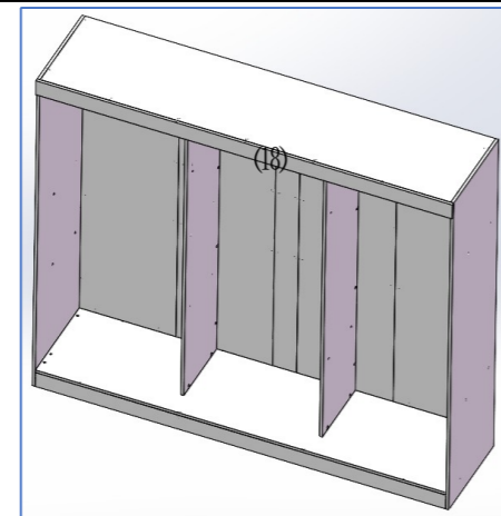
Board: (18) Screw: × 6
