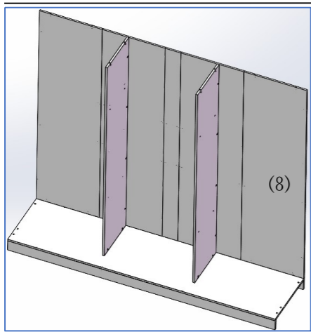
Board: (8) Screw: × 2 × 2
