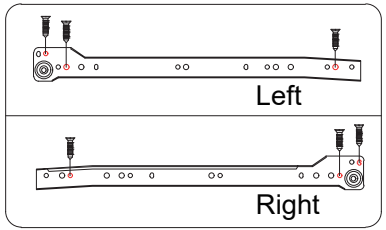
Right View
