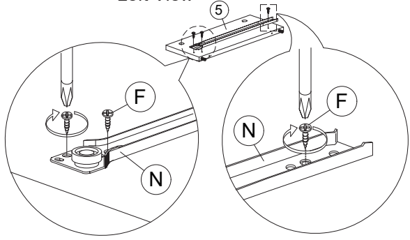
Left View
